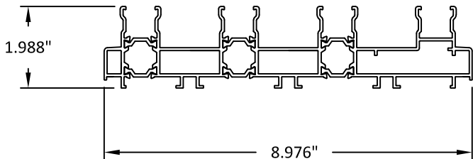
31 4 TRACK JAMB/HEAD/SILL 6063-T5/POLYAMIDE
