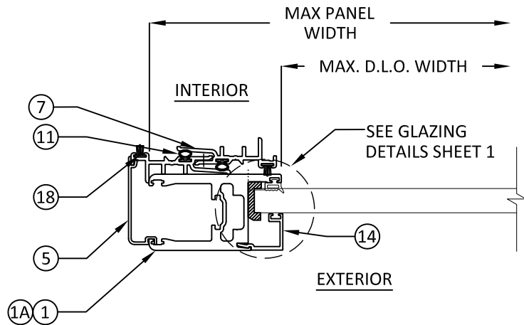
B 7 HORIZONTAL SECTION OUTSIDE POCKET WALL
