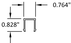
12 JAMB/HEADER TRIM 6063-T5
