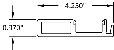
9 SASH/STILE INTERLOCK 6063-T5
