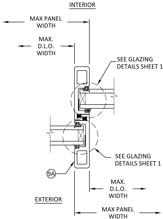
C 7 HORIZONTAL SECTION ALTERNATE INTERLOCK
