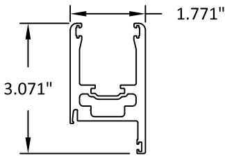
1 SASH RAIL/STILE 6063-T5
