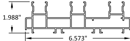
3A 3 TRACK JAMB/HEAD/SILL 6063-T5
