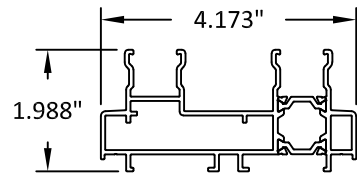
2 2 TRACK JAMB/HEAD/SILL 6063-T5/POLYAMIDE
