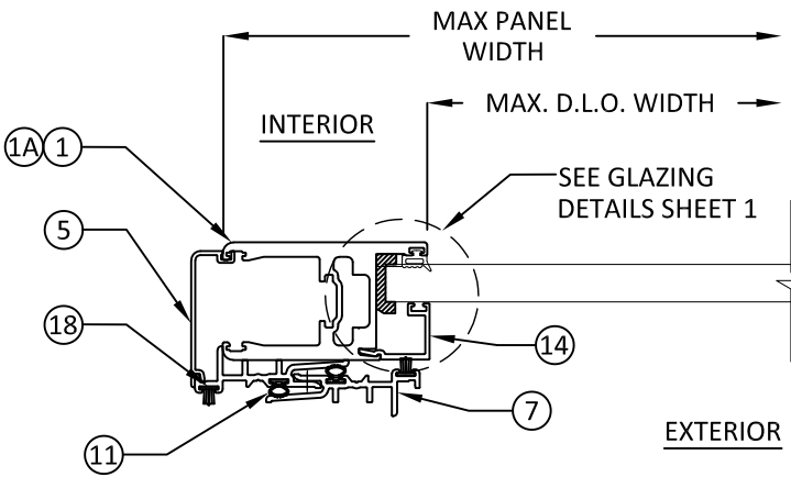
A 7 HORIZONTAL SECTION INSIDE POCKET WALL
