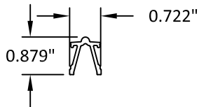
4 SNAP TRACK 6063-T5
